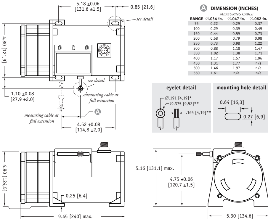
Fig. 2 – Outline Drawing (36 oz. cable tension only)
